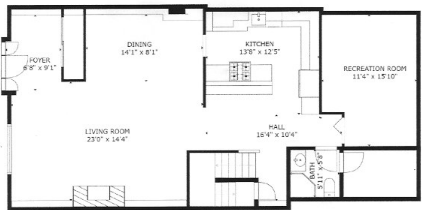
FLOOR 1
